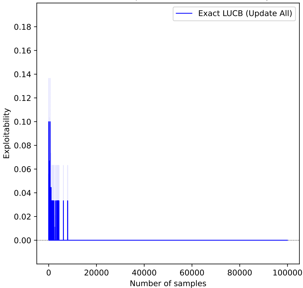
Kuhn Poker, PAC, \epsilon = 0.01 , \delta = 0.01 , Player x
